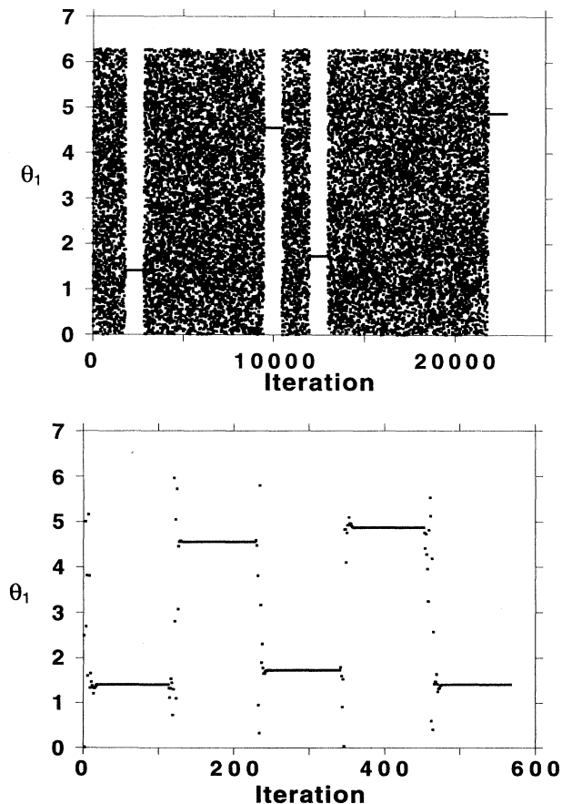
FIG. 2. Graphs illustrating switching between five different fixed points. The \theta_1 coordinate of the state is plotted versus iteration. In (a) we rely on ergodicity to bring the orbit close to the desired UPO. The fifth fixed point required 153 485 iterations to be stabilized, and is not shown. In (b), tree targeting is employed.
