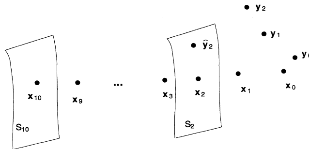
FIG. 3. Schematic diagram of the targeting procedure. Two successive perturbations of the kick are applied at \mathbf{y}_0 to steer it onto the stable manifold associated with the point \mathbf{x}_2 .
